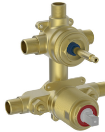
1/2" male NPT or welded copper connections
