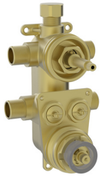
1/2" male NPT or welded copper connections
